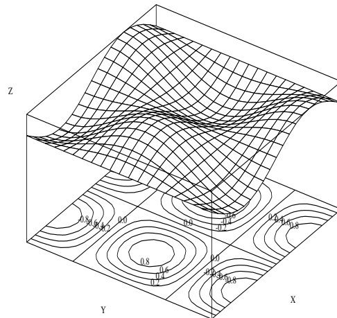
plot3d and contour
