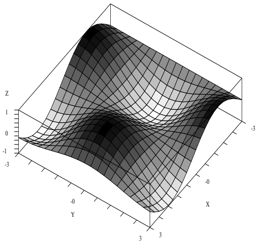
plot3d1 : z = \sin(x) \cdot \cos(y)
